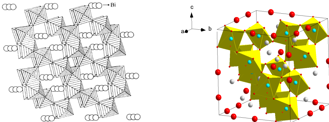
(v) \alpha\text{-Bi}_2\text{Ti}_4\text{O}_{11} ( C2/c ) [21]
